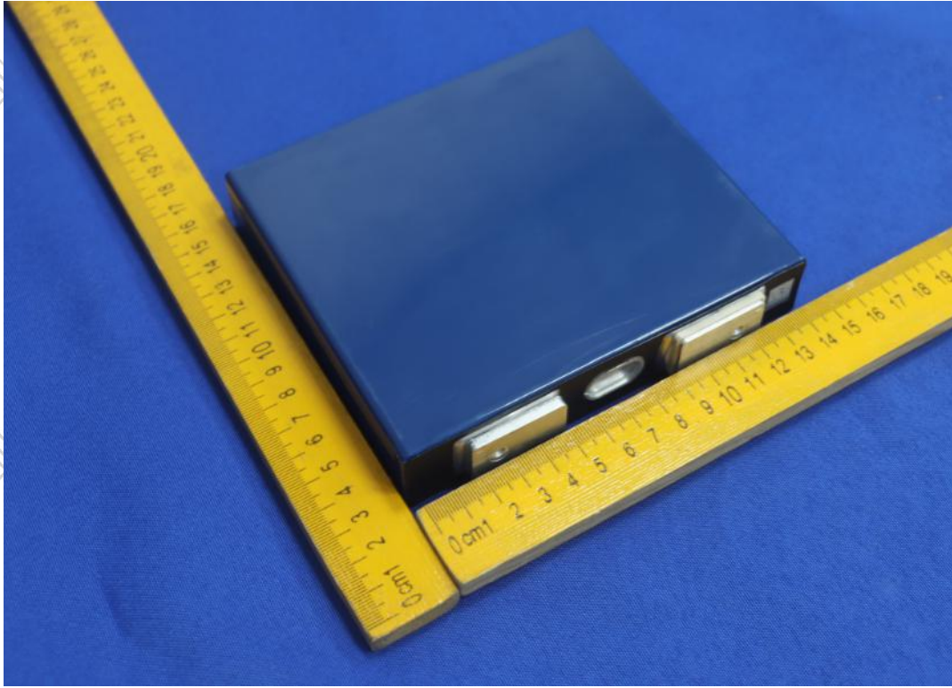
Figure 3 Overall view of cell (电芯图)
