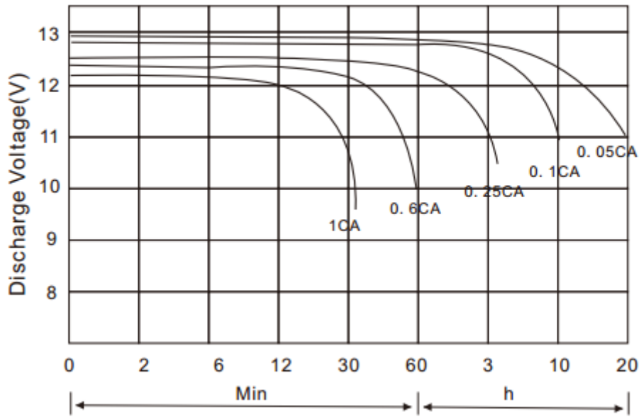
Fig.2-1. Discharge Curves at different current
