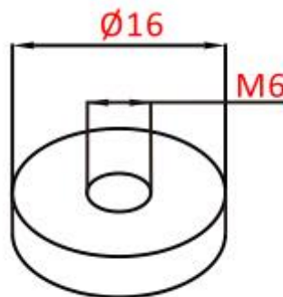
Terminal Dimensions
