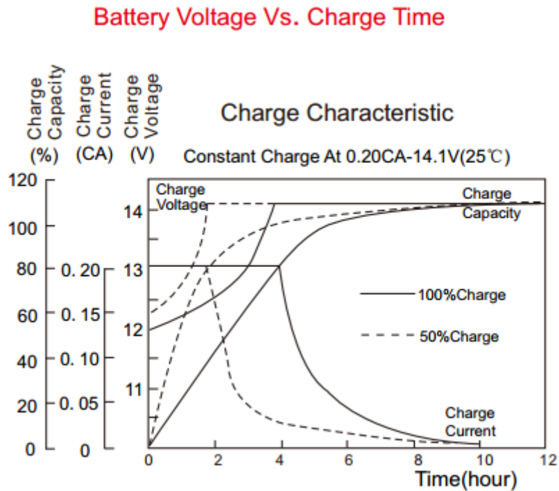
Fig.2-2. Charge Curves at 25 °C
