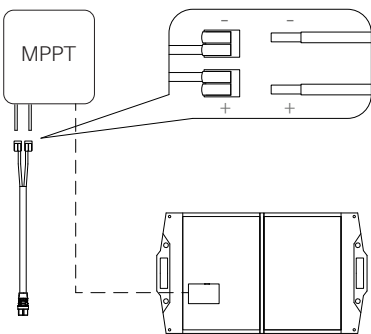
Connect with Other Matched PV Panel
